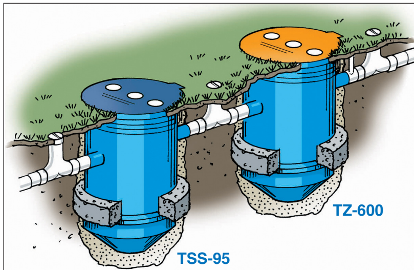
Trapzilla™ Model TSS-95 Solids Interceptor installed upstream of a TZ-600 Grease Interceptor
